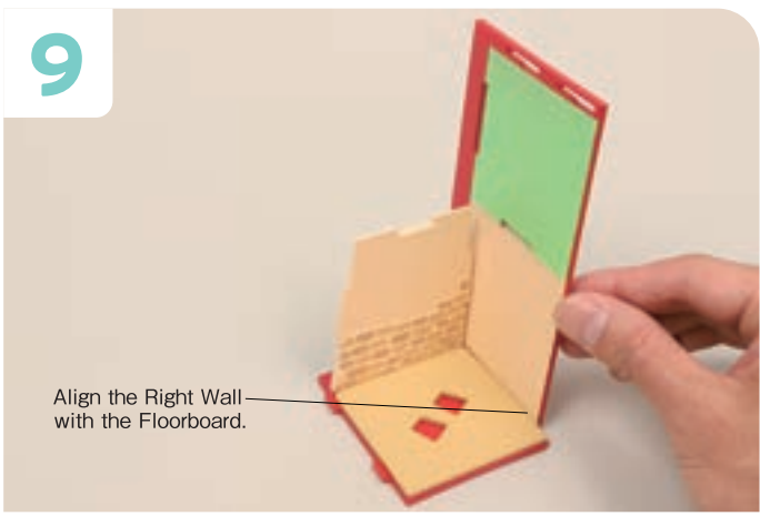
Insert the protrusions all the way into the holes and fit the Floorboard and Right Wall snugly.
